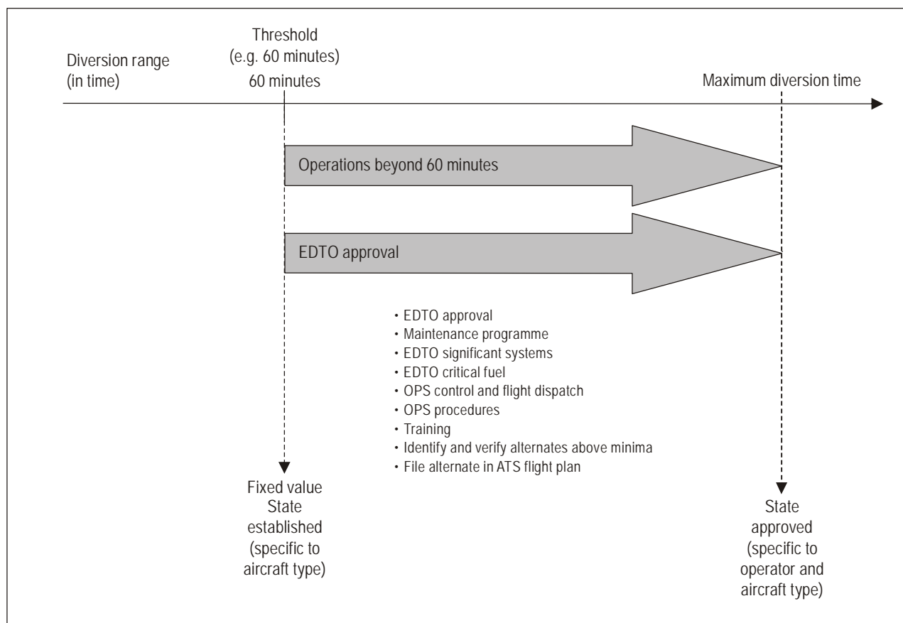
Figure D-7. Generic EDTO graphical representation for aeroplanes with two turbine engines
